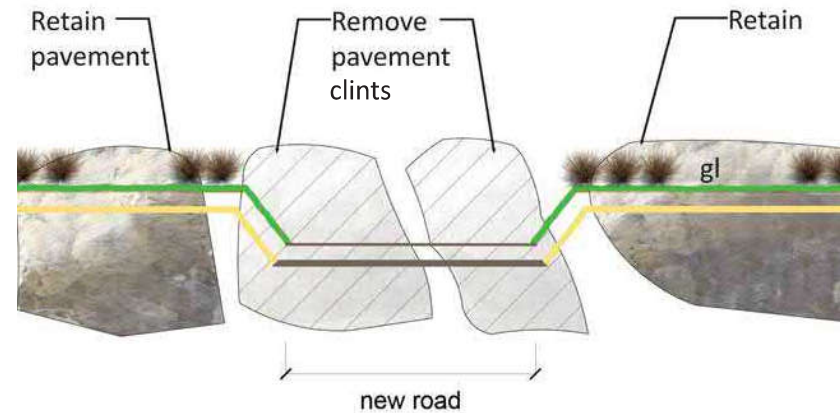
Fig. 53 Limestone pavement, showing clints, section.
