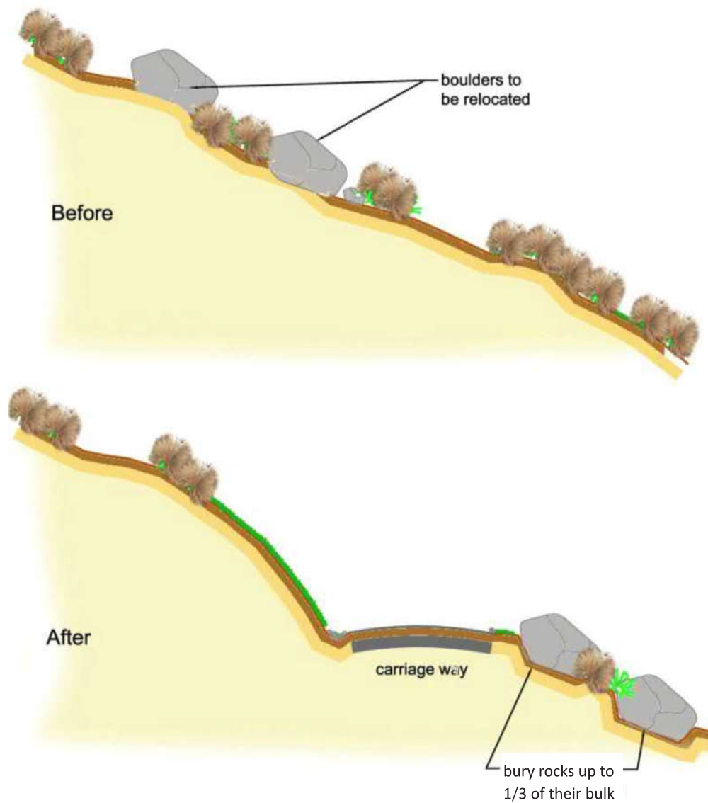
Fig. 16 Transfer boulders from uphill of the newly formed access road to below the road.
